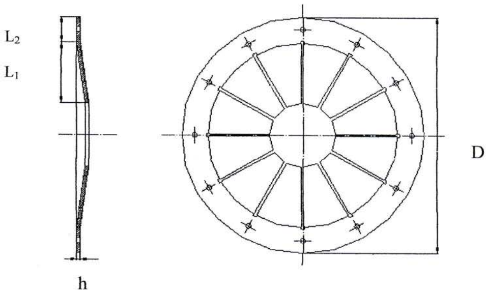
Gambar 8. 1. Pegas Matahari
