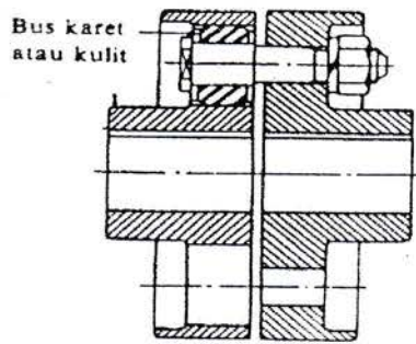
Gambar 2. 4. Kopling Flens Luwes
