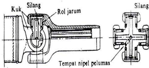
Gambar 2.9. Kopling Universal Hooks
