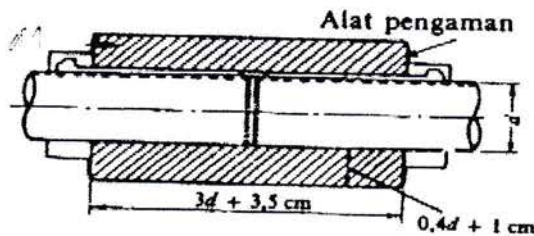
Gambar 2.1. Kopling Bus
