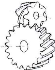
Roda Gigi Silang
