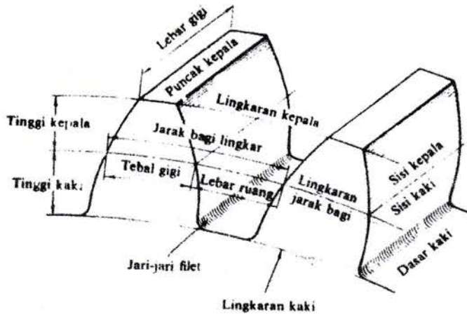
Gambar 3.Roda Gigi
